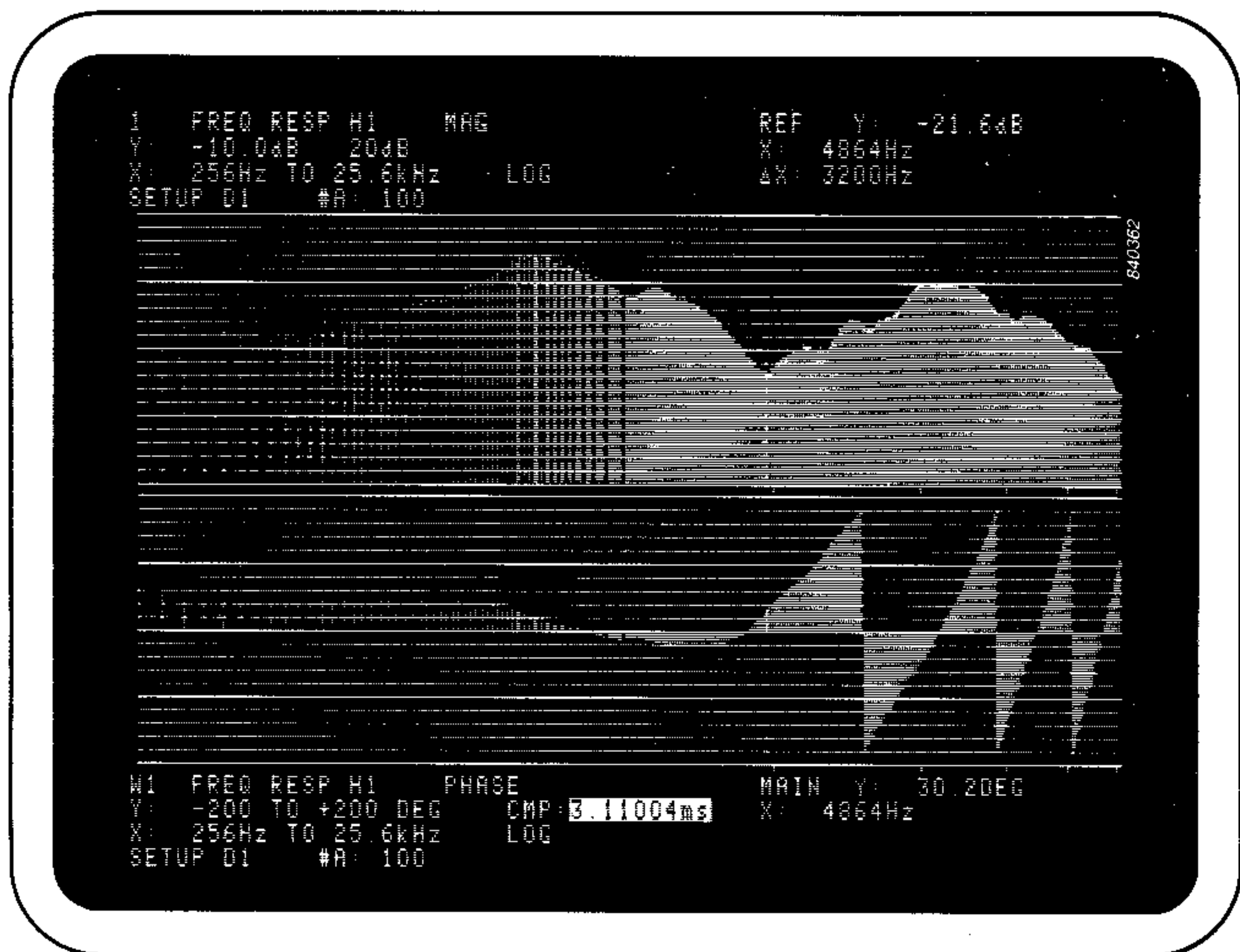
Fig. 6. The linear frequency response axis of Fig. 5, which is inherent to FFT-based analyzers, can be converted into a logarithmic axis, here showing the magnitude as well as the phase of the frequency response. Note that the phase has been compensated to take into account the delay ( \approx 3,11 ms) between the woofer and the measurement microphone
