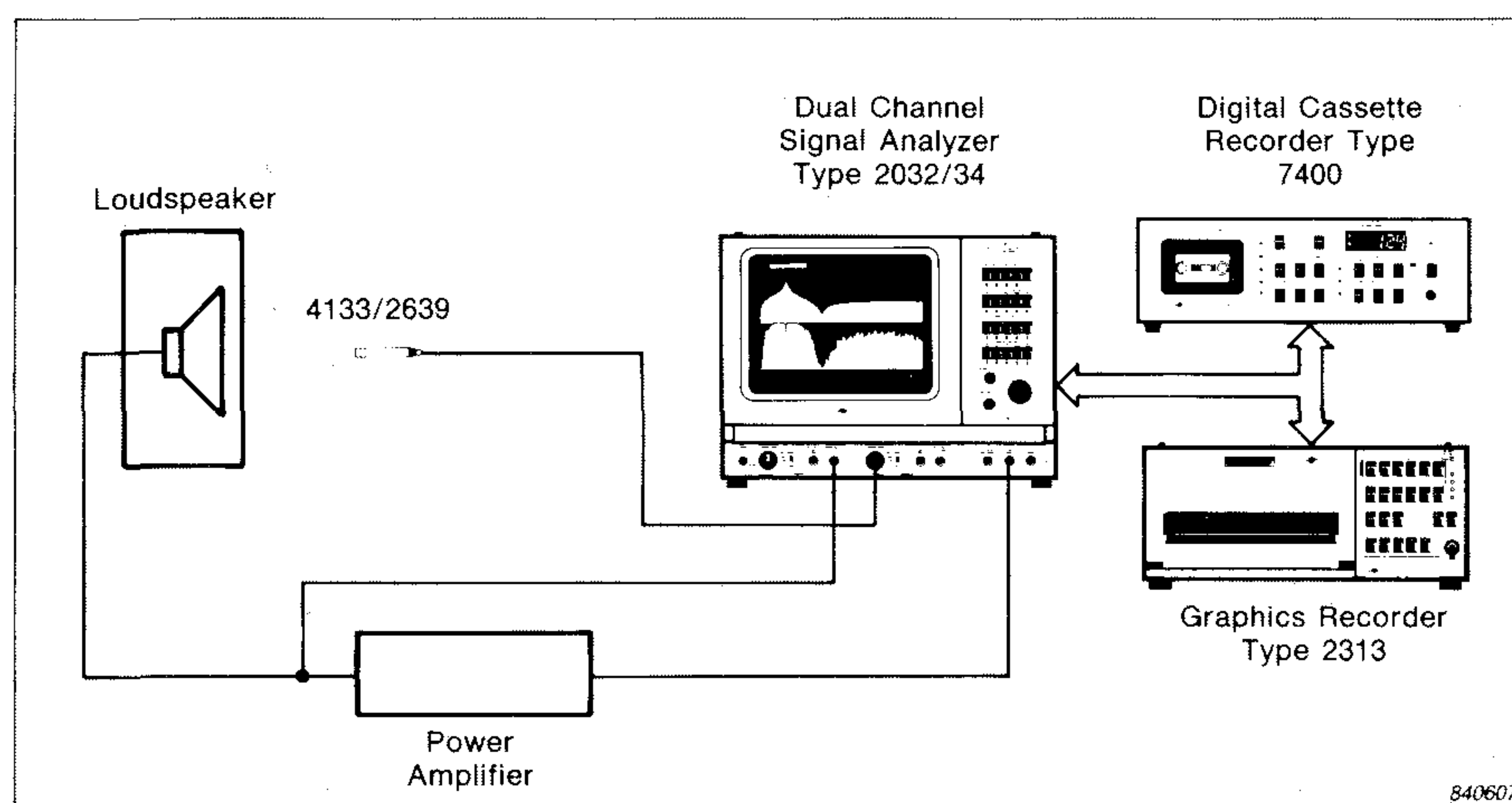
Fig. 1. General set-up for loudspeaker measurements. The Digital Cassette Recorder Type 7400 is used for storage of the measurement set-ups in addition to storage of the measured data. Graphics Recorder Type 2313 is used for reformatting data and for plotting results
