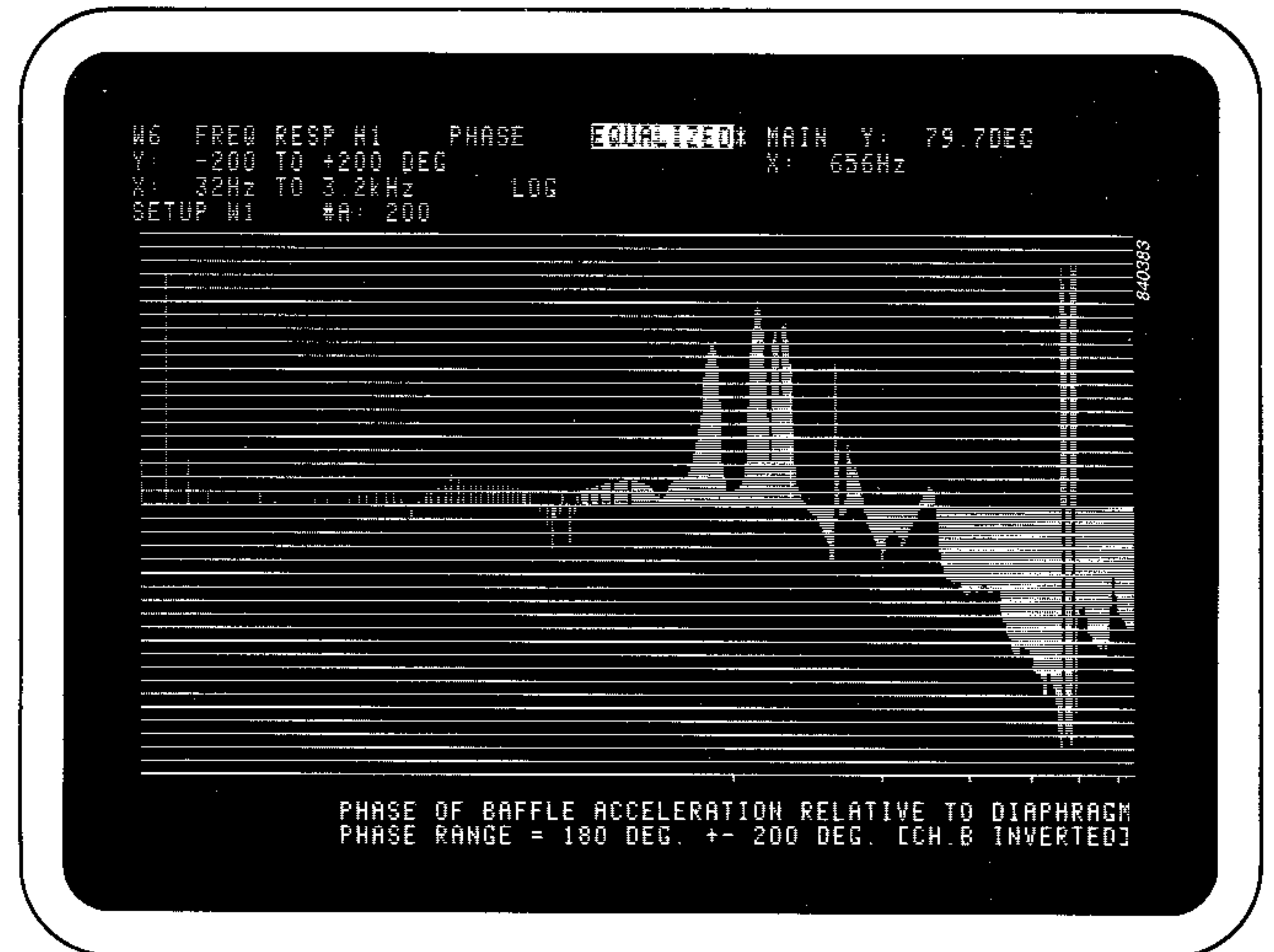
Fig. 19. Phase response corresponding to the lower curve of Fig. 18. In the low frequency range the phase of the baffle vibration is 180^\circ out of phase with the diaphragm movement. (Note: shifted phase range due to polarity reversal in channel B). This is a direct consequence of Newtons second law and a lack of mechanical isolation between the loudspeaker chassis and the front panel
