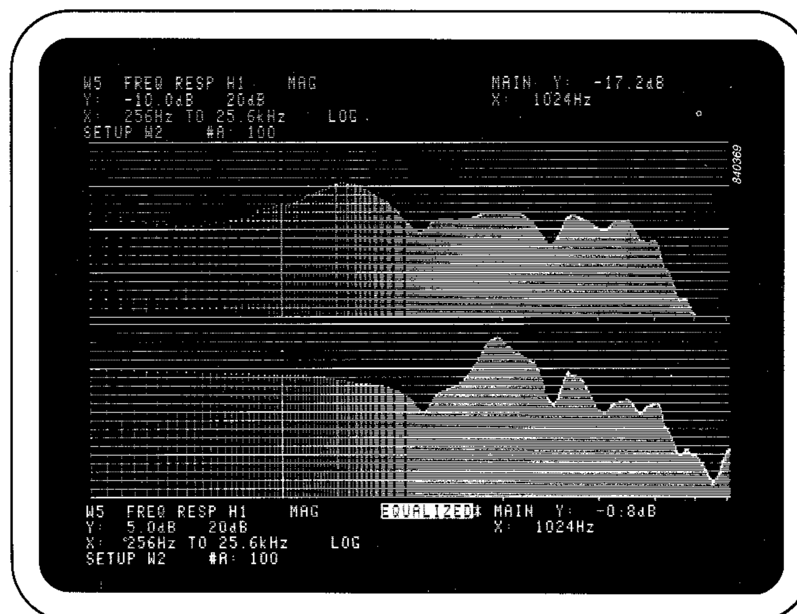
Fig. 11. The off-axis response in various directions will influence the degree of ambience in the reproduction.
