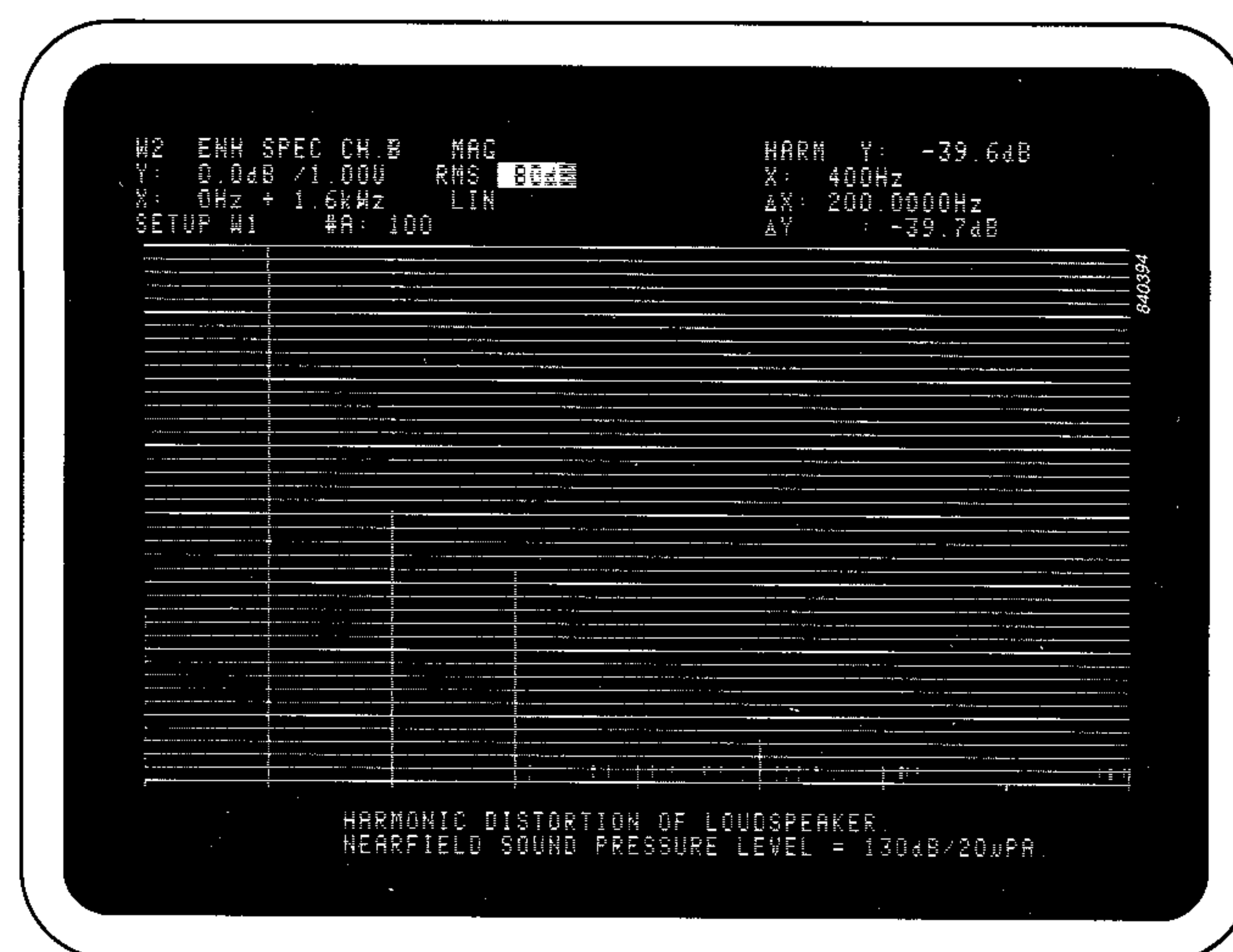
Fig. 25. Near-field measurement of harmonic distortion measured near the low frequency resonance of the loudspeaker. However, the sound pressure level should normally refer to the level at 1m distance from the loudspeaker. The cursor indicates a second harmonic distortion of -39,7dB relative to the fundamental
