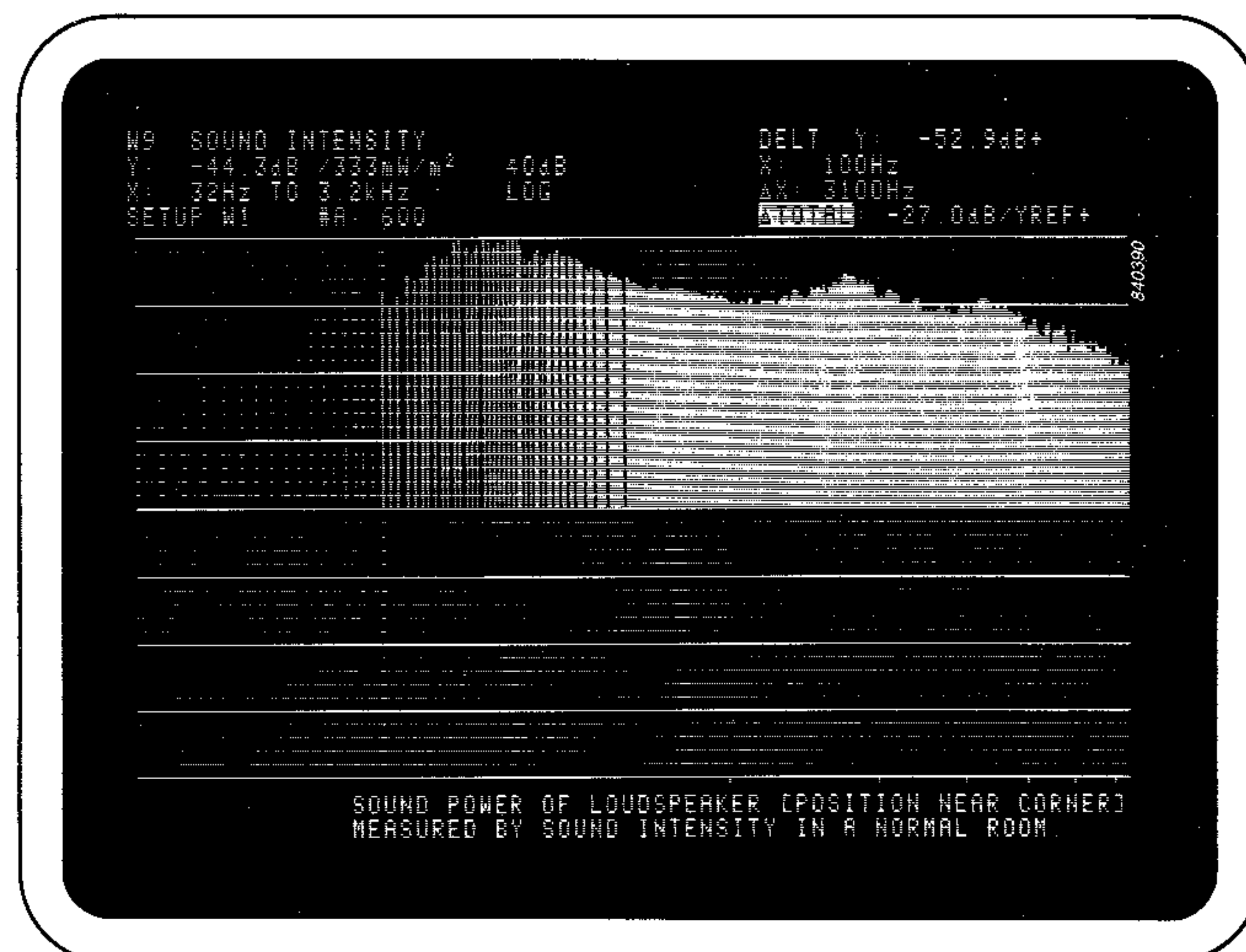
Fig. 23. Sound power measured as in Fig. 22, but with the loudspeaker positioned near a corner where the acoustical impedance better matches the radiation impedance of the speaker. This results in a higher acoustical output in the low frequency range. Due to the absorbing surfaces near the corner, the response in the upper part of the displayed range is lower than the response shown in Fig. 22
