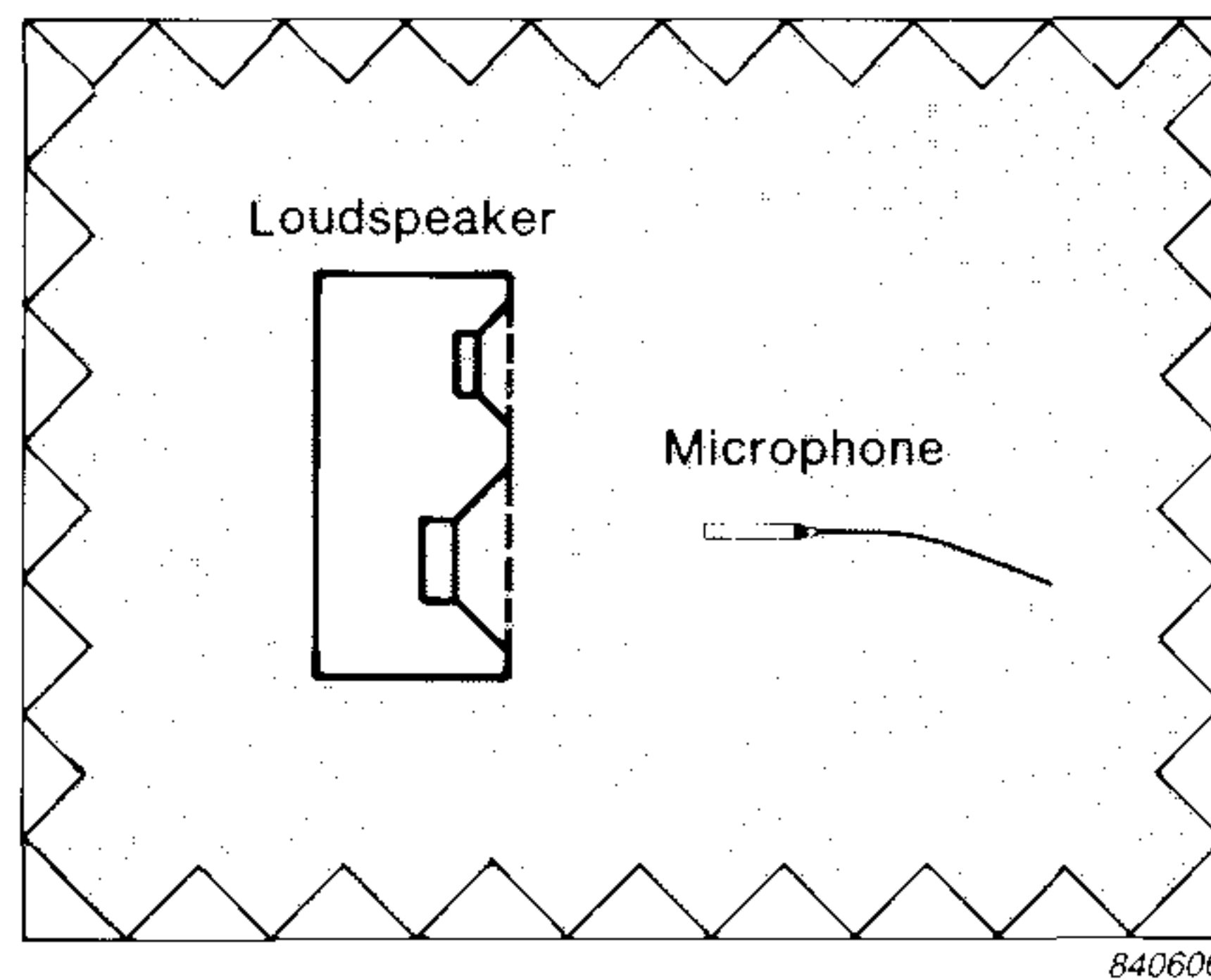
Fig.3. The on-axis free-field response is the most commonly used characteristic for the evaluation and documentation of transducer performance. Traditionally the direct sound is measured in an anechoic room, the boundaries of which absorb reflections and reverberant sound
