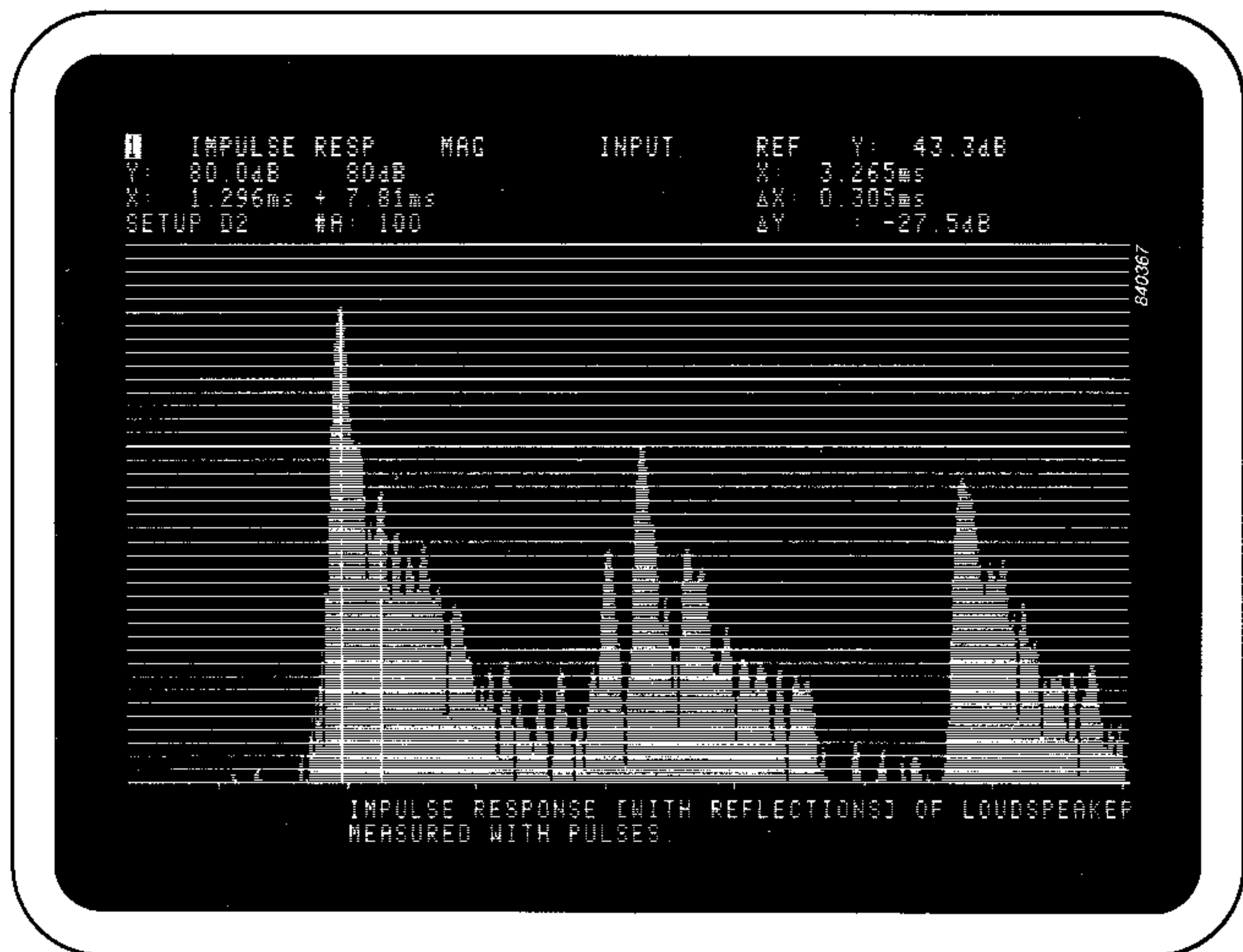
Fig. 9. Two reflective objects placed near the loudspeaker are easily identified on the impulse response display
