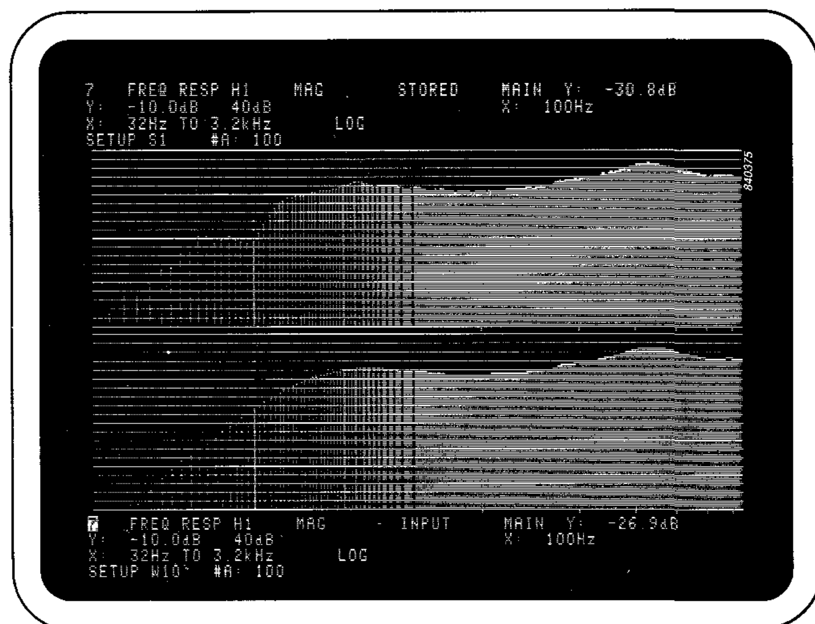
Fig.16. Low frequency free-field response of a small loudspeaker system measured in an anechoic room (upper curve) and using the impulse method in an ordinary room of equal dimensions (lower curve). The irregularities of the anechoic response seen around the cursor position are due to the presence of standing waves as the acoustical absorption at the room boundaries is not sufficient at these low frequencies.
