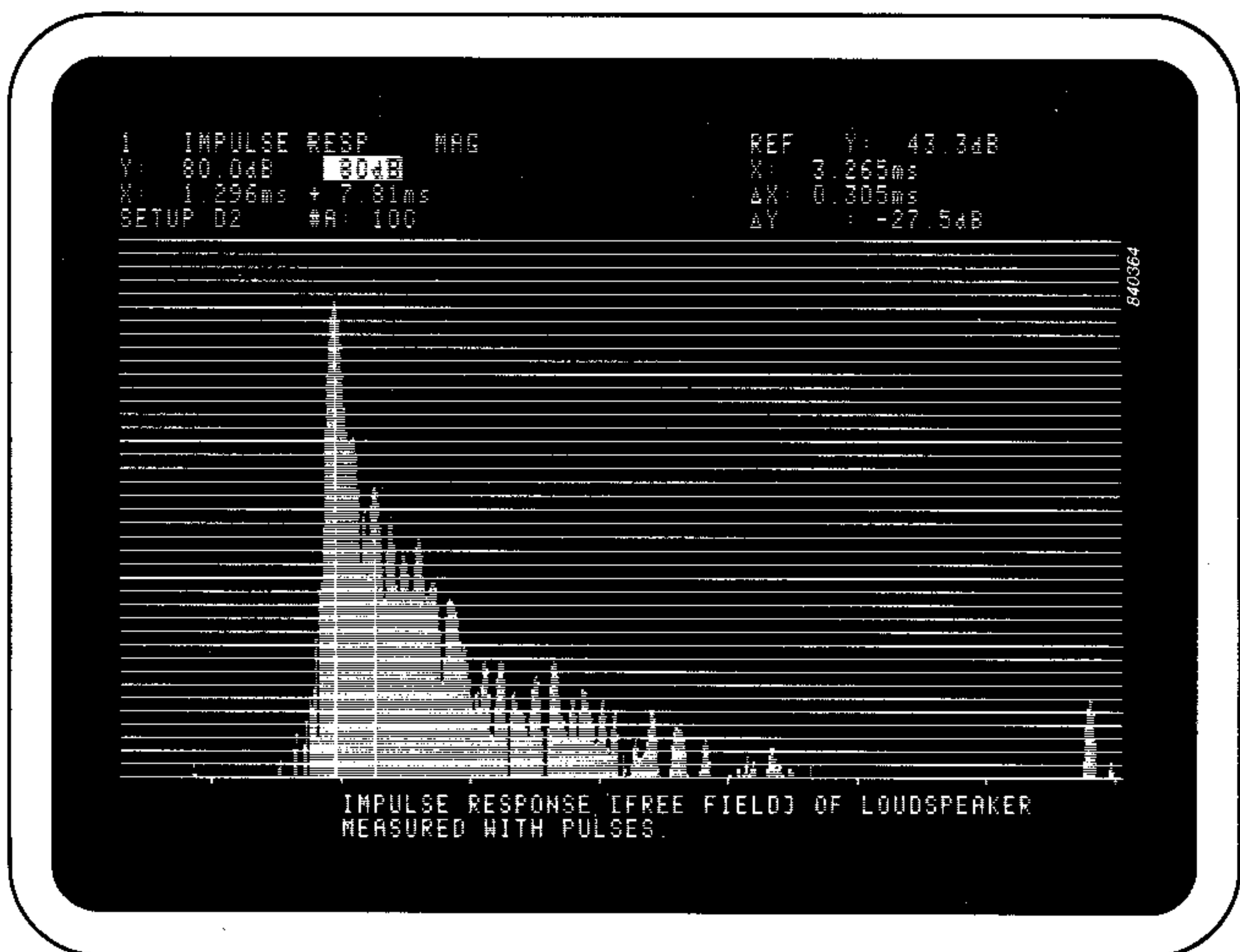
Fig. 8. Analyzers Types 2032 and 2034 allow logarithmic presentation of the impulse response magnitude. This feature vastly increases the possibilities for examination and correction of time domain discrepancies
