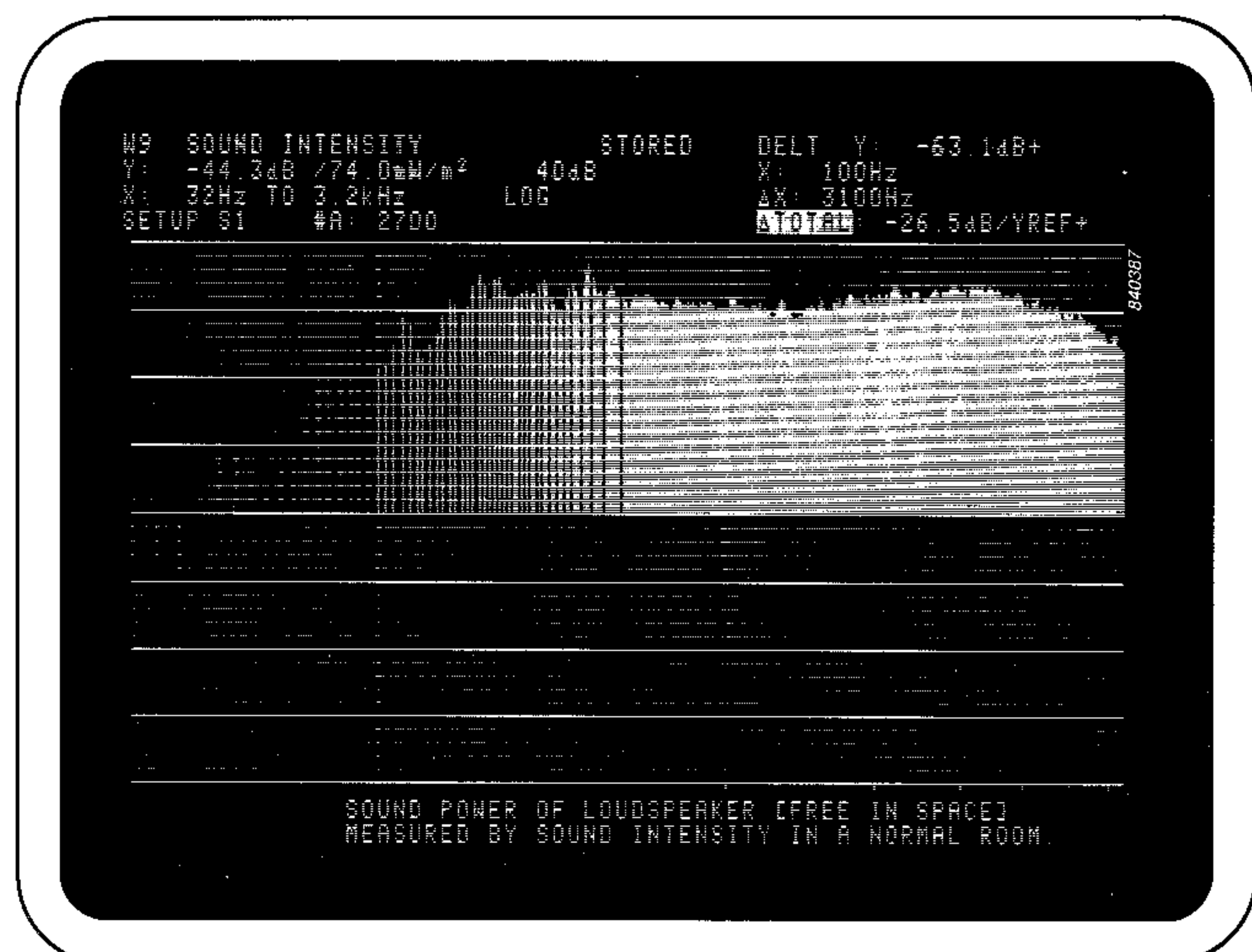
Fig. 22. Sound power output for 1W electrical input. The sound power is measured by averaging the sound intensity at 54 positions on a cube ( 4\pi steradians) around the loudspeaker in an ordinary room. With the probe configuration used, the measurement results are valid at frequencies down to approximately 100Hz. Measurement at lower frequencies requires a larger gap between the two microphones in the probe. Response below the centre horizontal axis indicates a negative intensity
