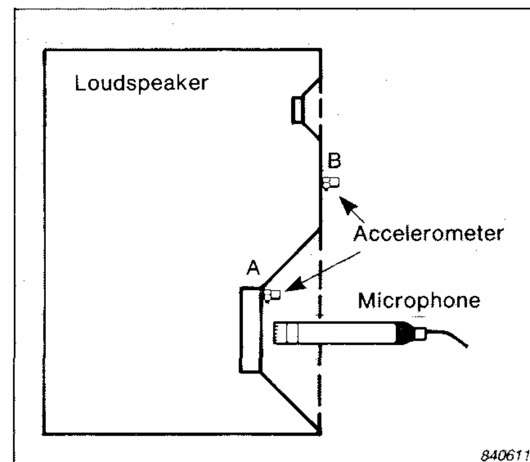
Fig.15. For the measurement of the near-field response, the microphone should be placed near the centre of the diaphragm. Cabinet vibration is measured by placing a small accelerometer at various positions on the loudspeaker cabinet. Measurement of the acceleration near the joint between the voice coil and the diaphragm can be used as a reference
