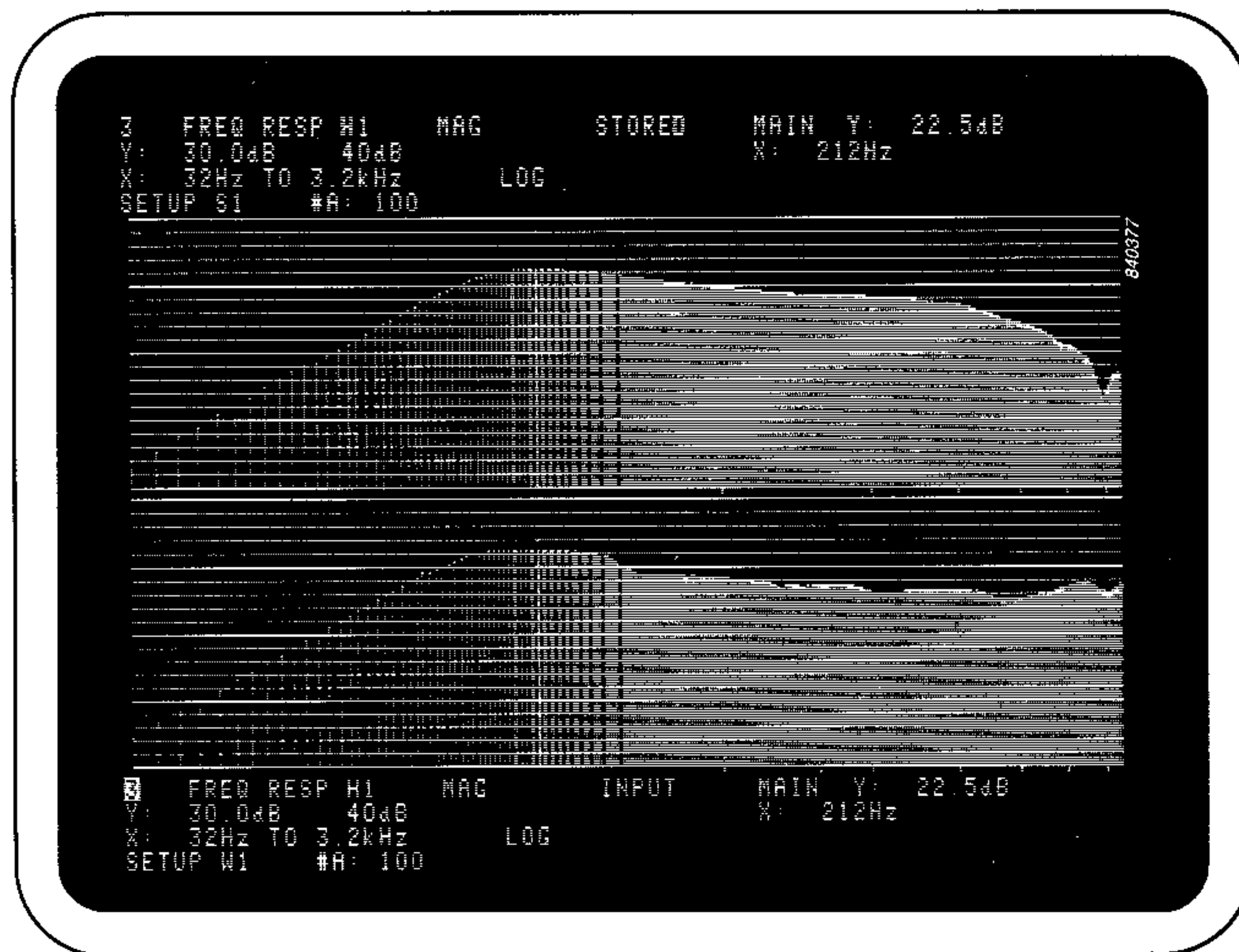
Fig.17. Near-field response (upper curve) and diaphragm acceleration (lower curve) of the same loudspeaker used for the measurements in Fig.16. With the near-field technique there is no low frequency limit. The measured response shows good agreement with the free-field response for frequencies up to approximately 600Hz. Below 300 Hz the diaphragm acceleration is seen to be directly proportional to the near-field response, indicating that in this frequency range the diaphragm behaves like a rigid piston
