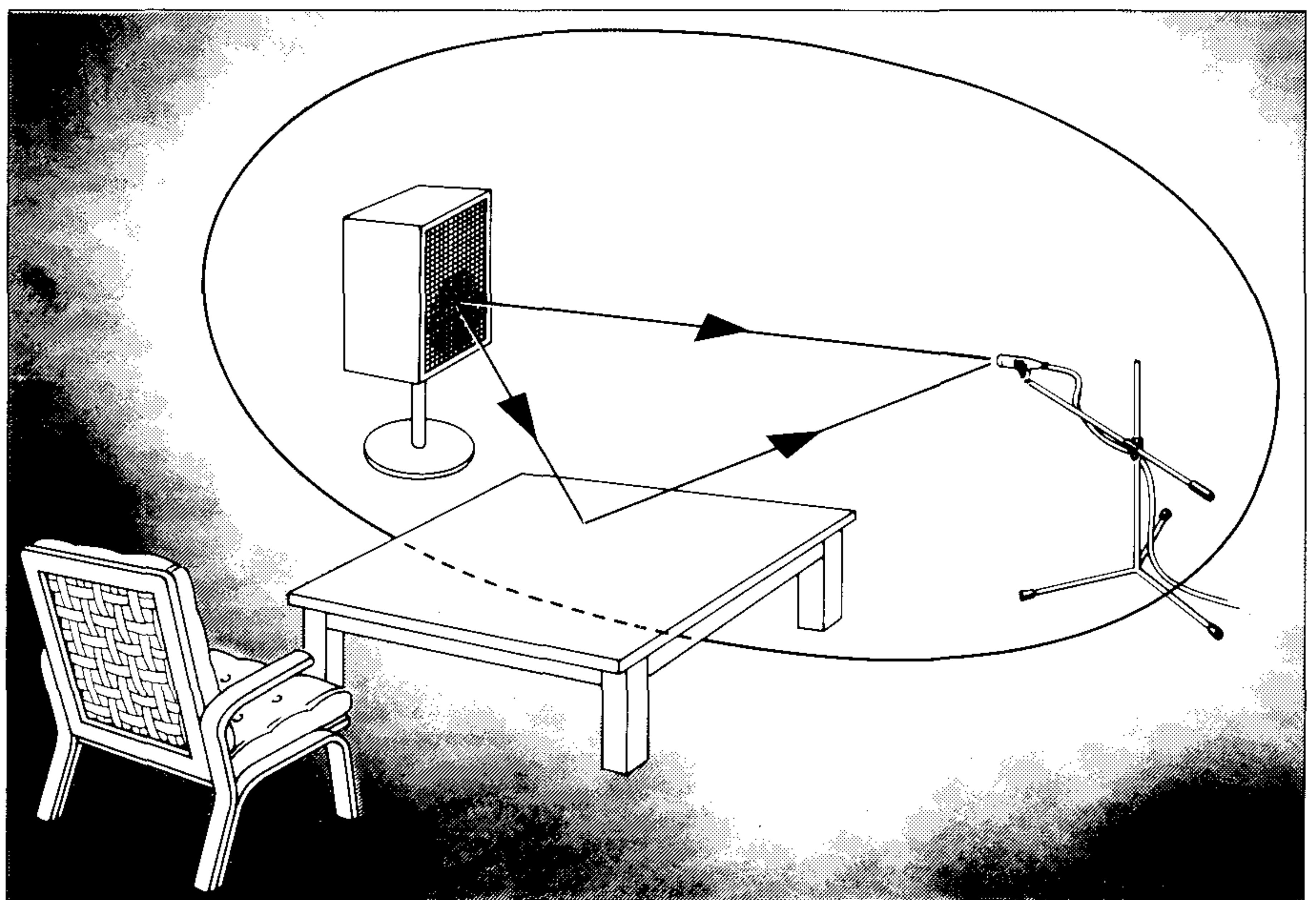
Fig.4. When the measurement technique allows the use of time gating — windowing — it is possible to isolate the direct sound from the reflections which are always present in a normal environment. Only objects which are located within an ellipsoid, the size of which depends on the length of the time window, interfere with the measurement
