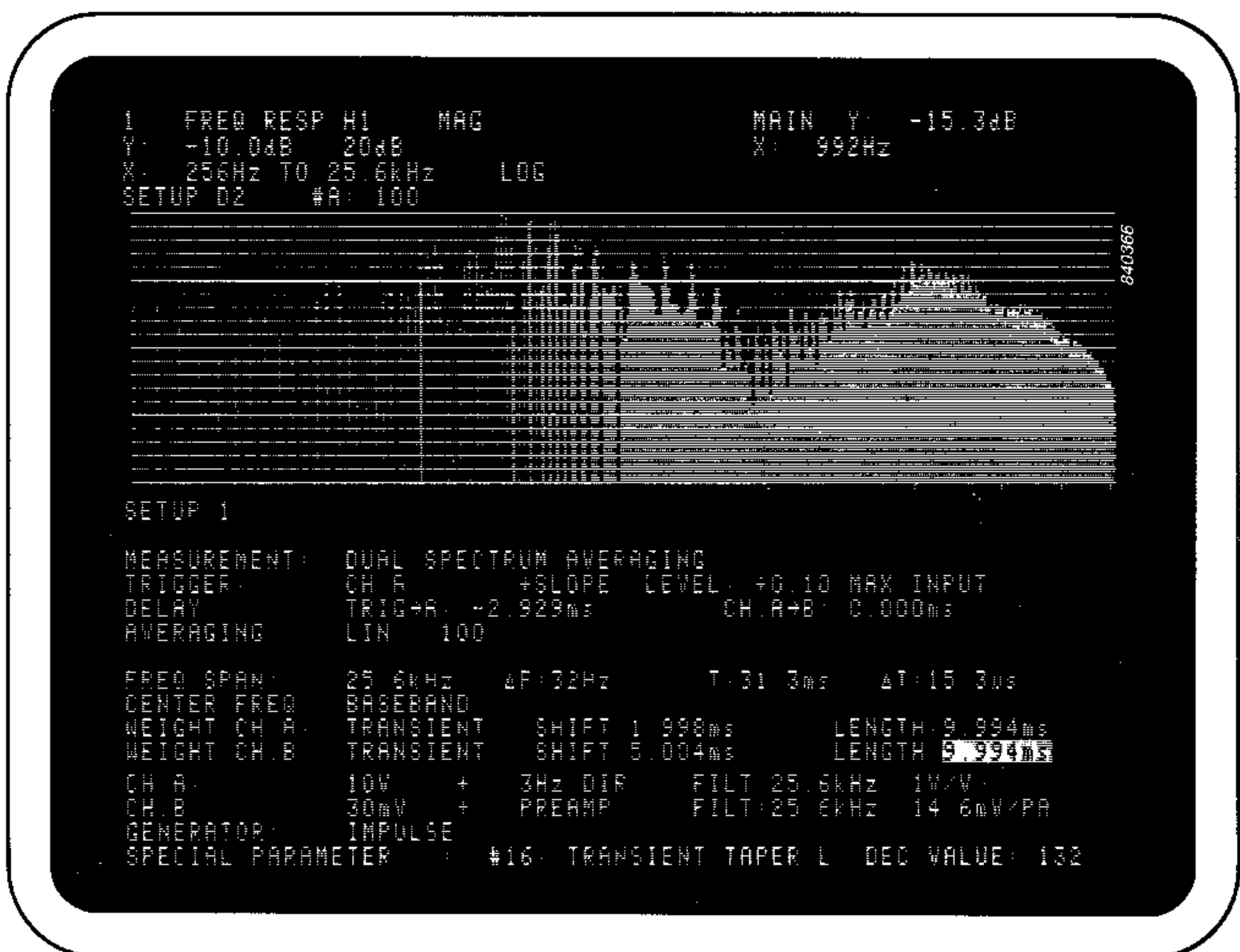
Fig. 10. From the frequency response corresponding to Fig. 9., however, it is more difficult to disclose the actual cause of the response irregularities
