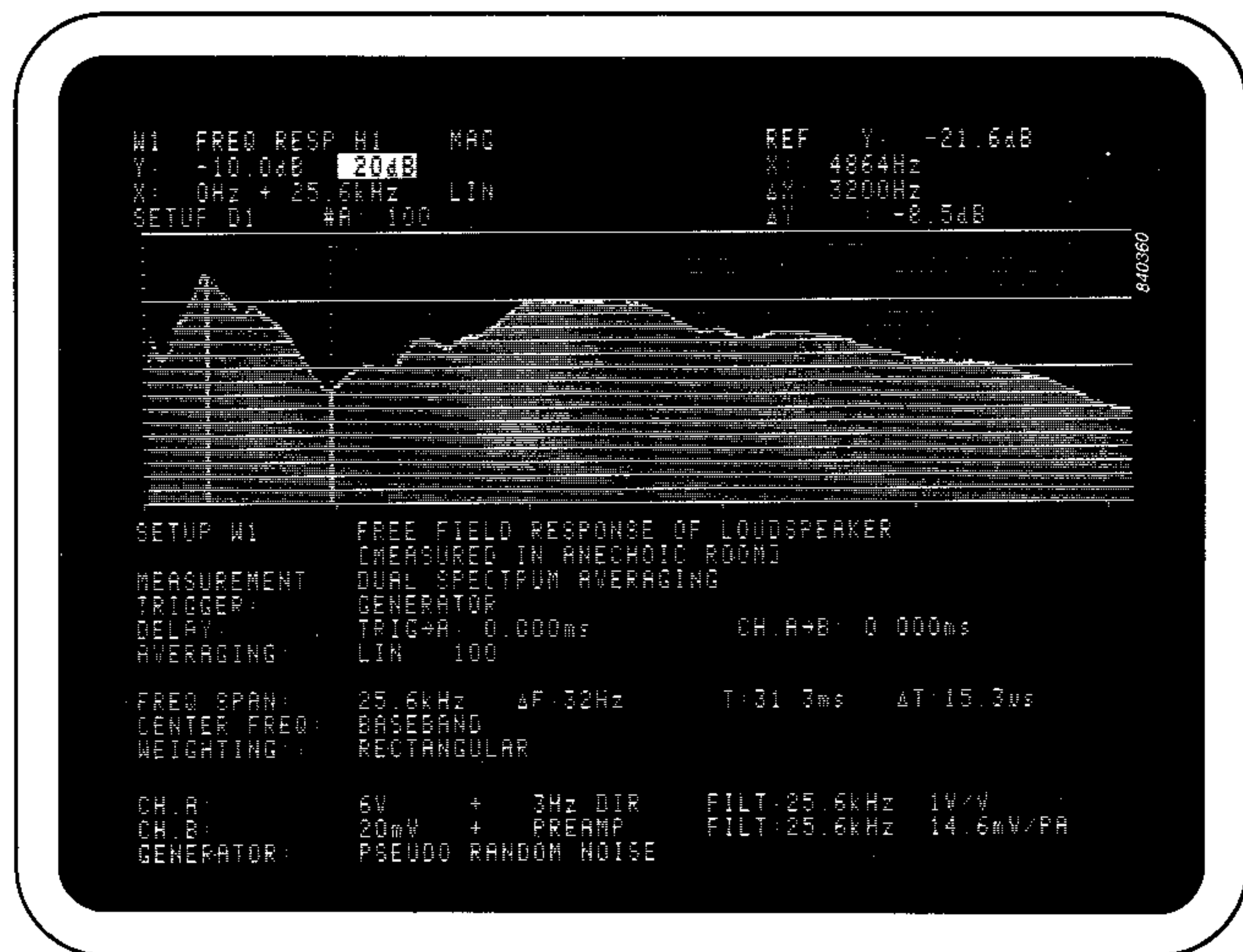
Fig. 5. The free-field response of a loudspeaker measured with pseudo-random noise excitation in an anechoic room. With this periodic type of white noise, the measurement converges more quickly towards the actual response than with true random noise excitation. The reference cursor has been set to display the maximum level fluctuation of the response
