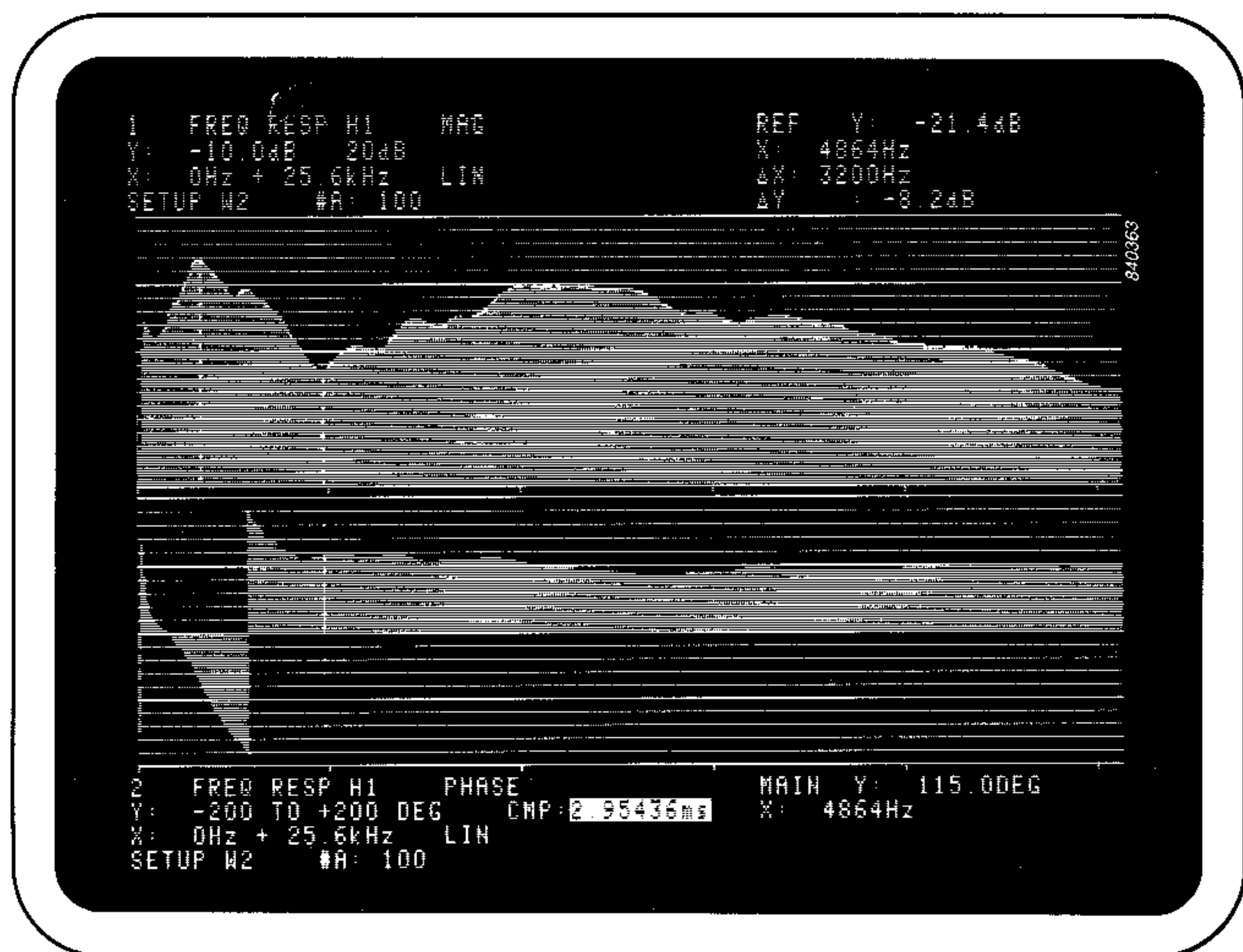
Fig. 7. Free-field response (magnitude and phase) of the same loudspeaker, but measured with the time selective impulse technique. The phase response has been compensated to account for the delay of the tweeter ( \approx 2,95 ms). Displayed with a linear frequency axis, an offset in delay corresponds to a simple tilt of the phase response
