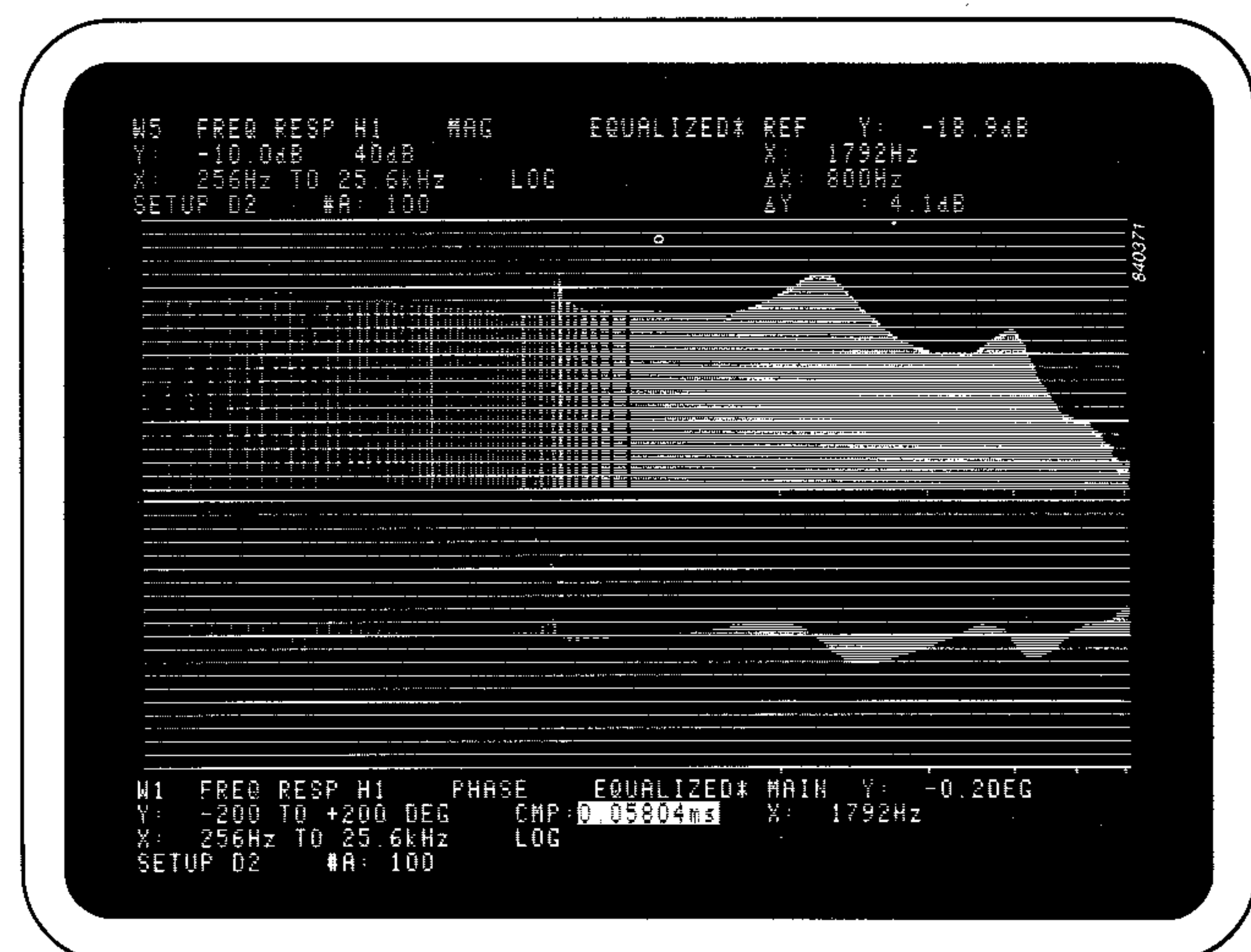
Fig. 13. The response of a microphone can be measured accurately by mere substitution of the test microphone for the measurement microphone used for the loudspeaker measurements. Using the equalized mode, the magnitude as well as the phase of the microphone response are compensated to account for the non-ideal response of the loudspeaker
