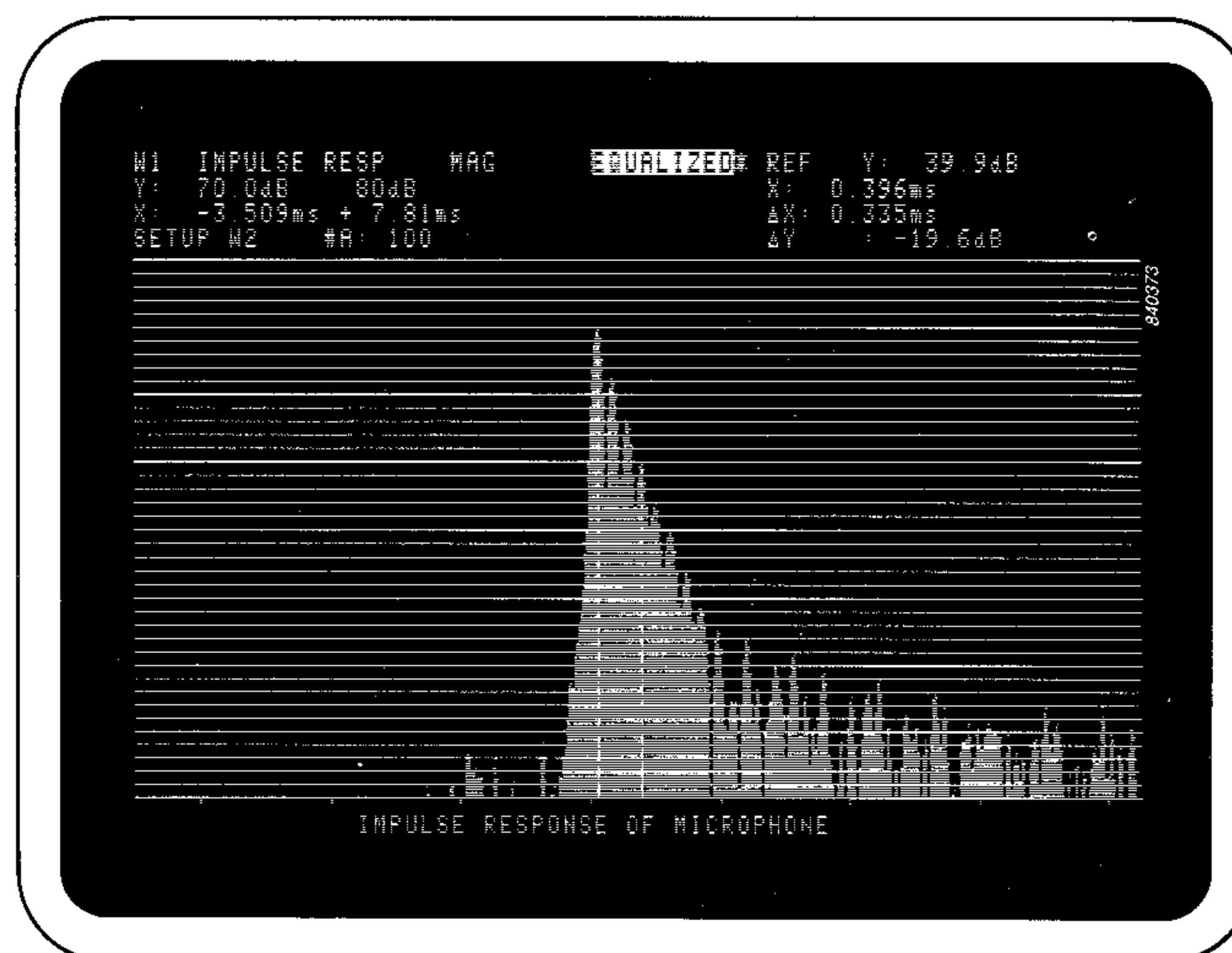
Fig. 14. Since the impulse response is obtained from the calculated frequency response rather than directly from the input data, it is also possible to extract the impulse response of a microphone from the combined response of loudspeaker and microphone. The logarithmic presentation provides direct visualization of the decay rate for the multiple reflection
