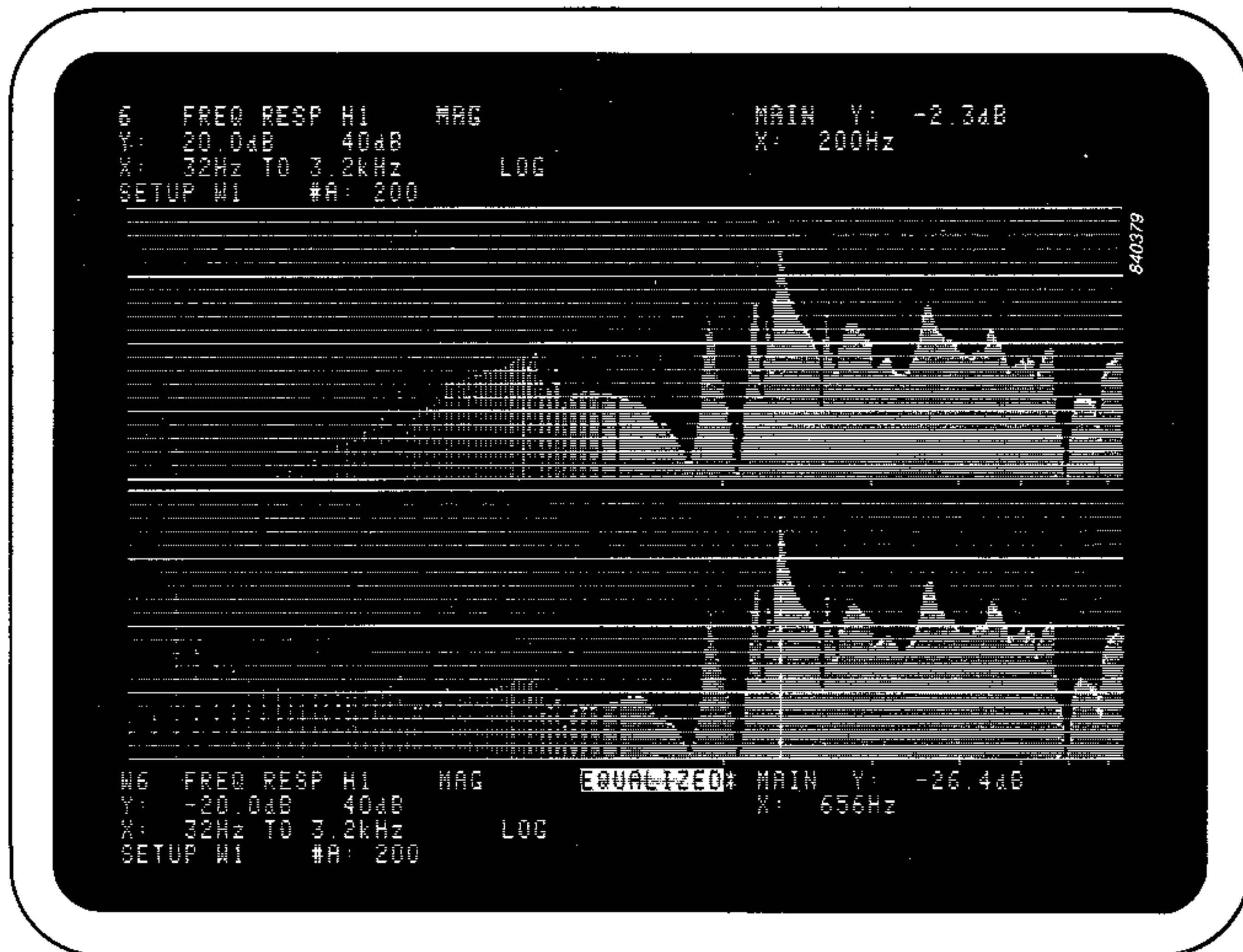
Fig. 18. Absolute level of front baffle vibration (upper curve) and baffle vibration relative to diaphragm movement (lower curve). Since the sound pressure resulting from this vibration is proportional to the vibrating surfaces, colouration related to cabinet vibration is generally a more severe problem with loudspeakers with large panel areas
