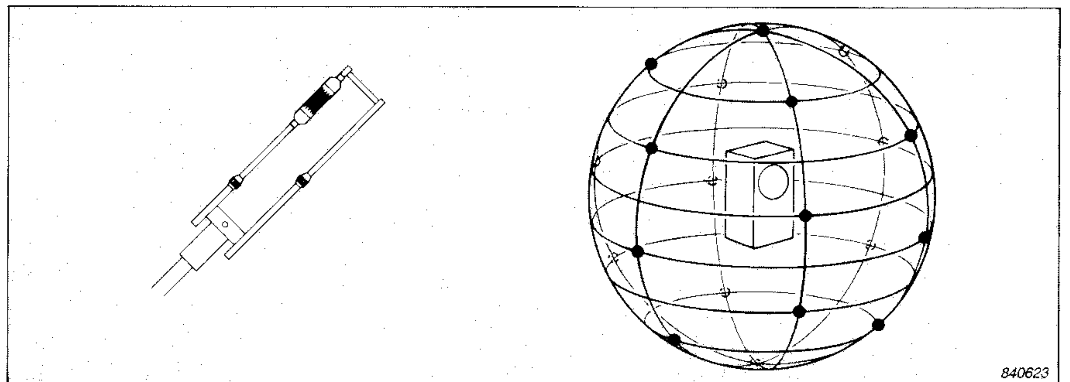
Fig. 20. To estimate the total sound power output of a loudspeaker, the sound intensity probe (left), or in the case of measurement in an anechoic room the measurement microphone, must be moved to a large number of positions on a hypothetical surface surrounding the loudspeaker. For an equal number of averages at each position these should represent areas of equal size (right)
