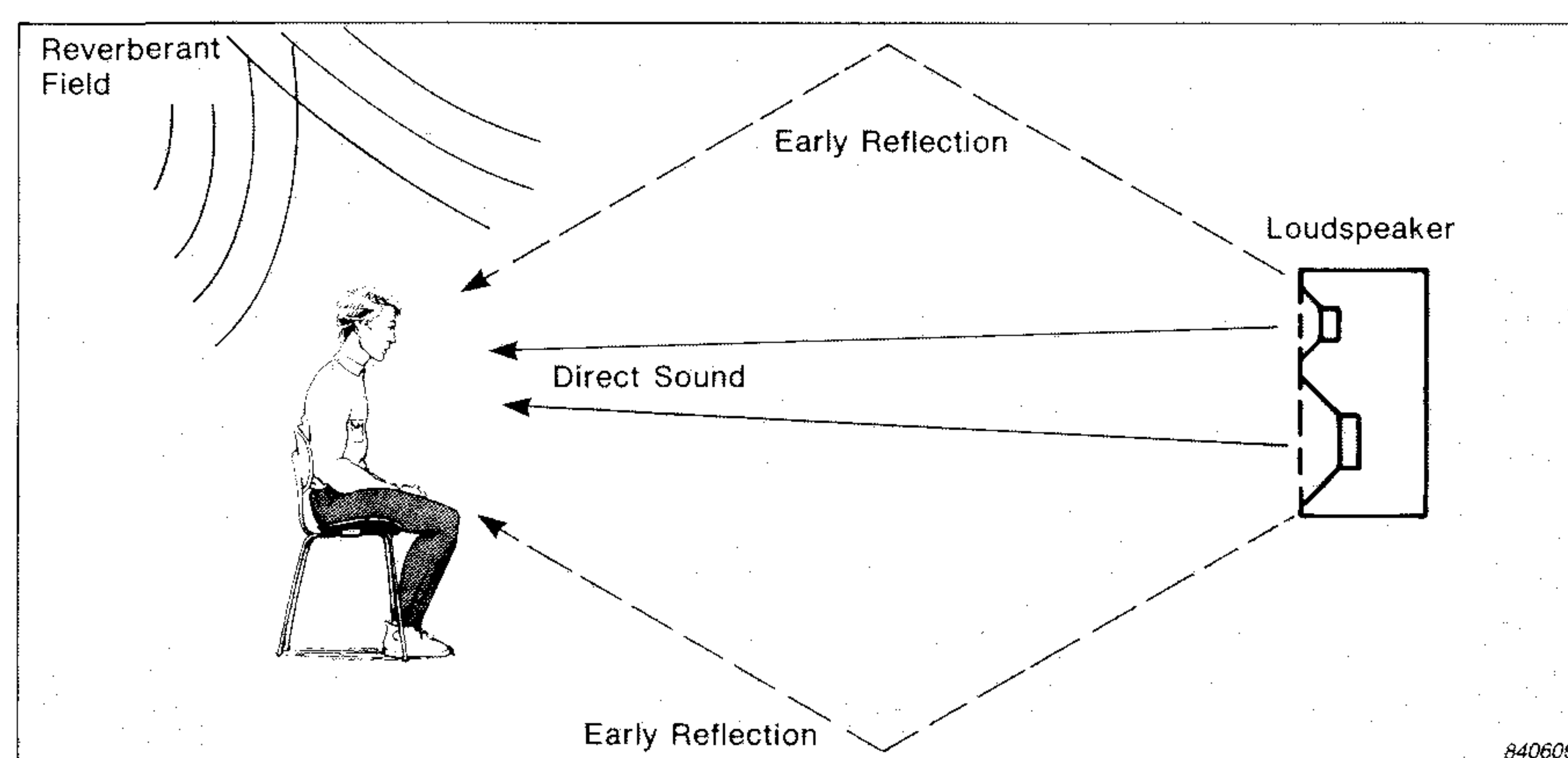
Fig. 2. In a practical listening situation, the interface between loudspeaker and listener is very complex. For convenience, contributions to the total sound field are often divided into three categories: the direct sound, the early reflections and the reverberant field
