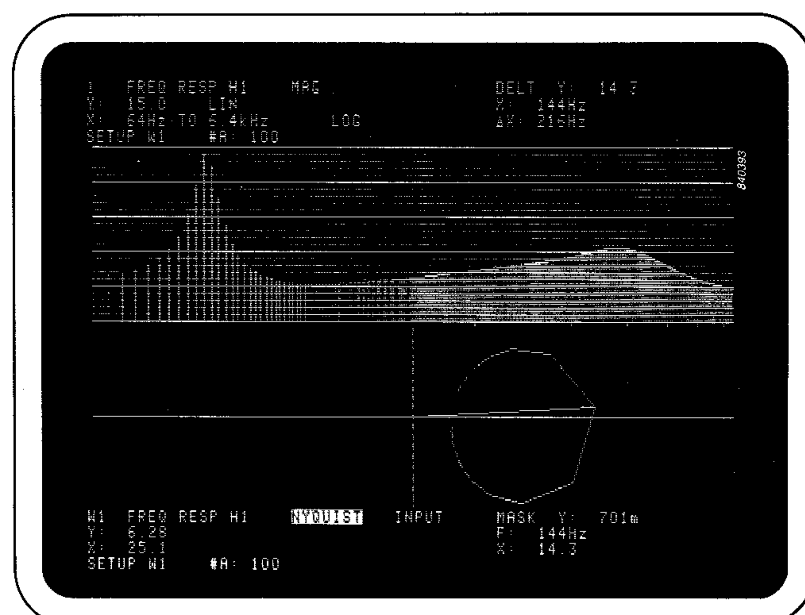
Fig. 24. Linear magnitude and Nyquist plot of loudspeaker impedance. A large (800 line) Fourier Transform is essential for obtaining an adequate resolution for simultaneous measurement of both resonance peaks. The "MASK" cursor used with the Nyquist plot helps eliminate the confusion often associated with such plots. The trace represents the frequency range indicated by the delta cursor in the upper display. Each resonance peak in the impedance plot will correspond to a full circle in the Nyquist plot
